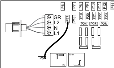
240V Convertible Connection
