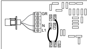
2-Phase Connection
