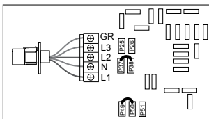
3-Phase Connection with Single Neutral
